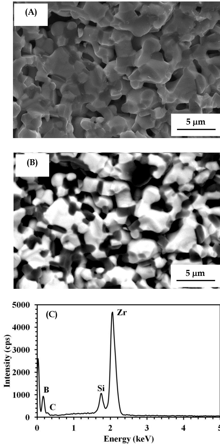
Figure 4.6: Micrographs and EDS analysis of \text{ZrB}_2\text{-SiC} inner bulk fractured cross-section after laser treatment (70 W). (A) Secondary electrons mode (SE) (4000 \times ), (B) Backscattering electrons mode (BSE) (4000 \times ) and (C) EDS spectrum of (B).
