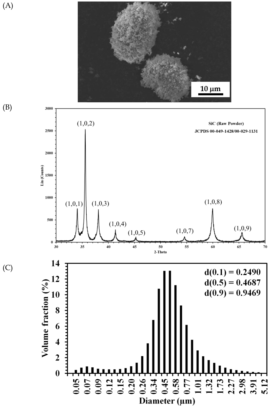
Figure 3.1: Analysis of SiC raw powders. (A) SEM micrograph (2000×), (B) XRD pattern and (C) Particle size distribution.
