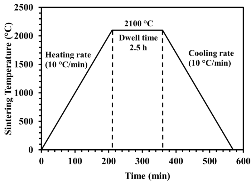
Figure 2.4: The sintering program at 2100 °C.
