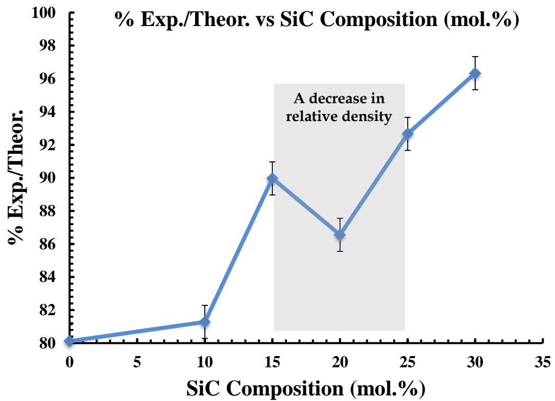
Figure 5.1: Percentage of experimental/theoretical density measurement of sintered pellet versus SiC composition (mol.%).
