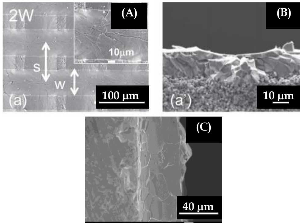
Figure 1.6: SEM images (A) Surface image of \text{TiO}_2 at 2 W, (B) Cross-sectional of \text{TiO}_2 at 2 W, and (C) Cross-sectional of ZnO irradiated at 126 W (Kido et al., 2011; Kido et al., 2014a).
