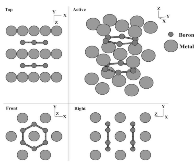
Figure 1.9: Schematic \text{ZrB}_2 crystal structure (Fahrenholtz et al., 2007; Li et al., 2010; Lonné, 2011).
