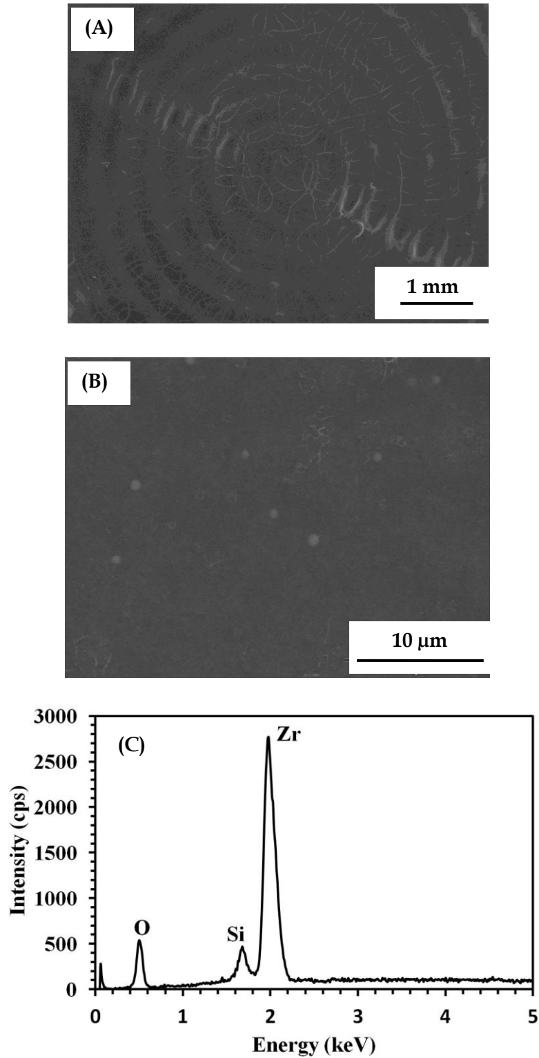
Figure 4.3: SEM micrographs and EDS analysis of \text{ZrB}_2\text{-SiC} surface after laser treatment performed at 70 W. (A) Low-magnification SEM image (20 \times ), (B) High-magnification SEM image (4000 \times ) and (C) EDS analysis of white spherical particles.
