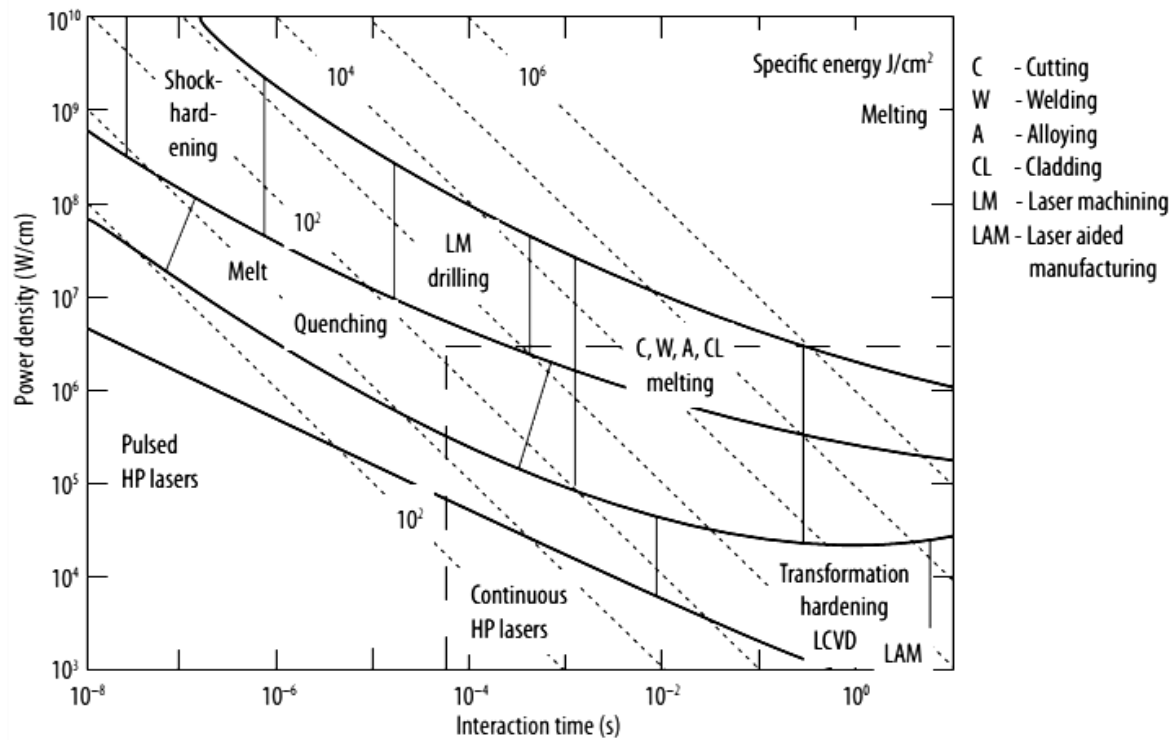
Figure 1.2: Operational regimes for various processing techniques. high-powered (HP), laser chemical vapour deposition (LCVD) (Steen & Mazumder 2010).
