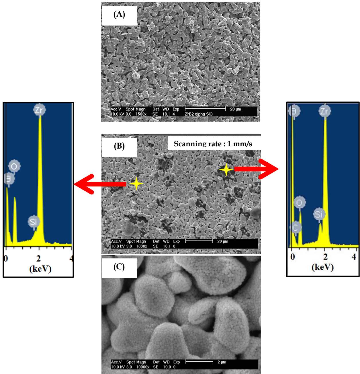
Figure 3.6: Secondary electron images of the transformation of sintered pellet of \text{ZrB}_2\text{-SiC} after laser treatment. (A) Sintered pellet (1500 \times ), (B) Laser-treated pellet (1000 \times ) and (C) High-magnification (10000 \times ).
