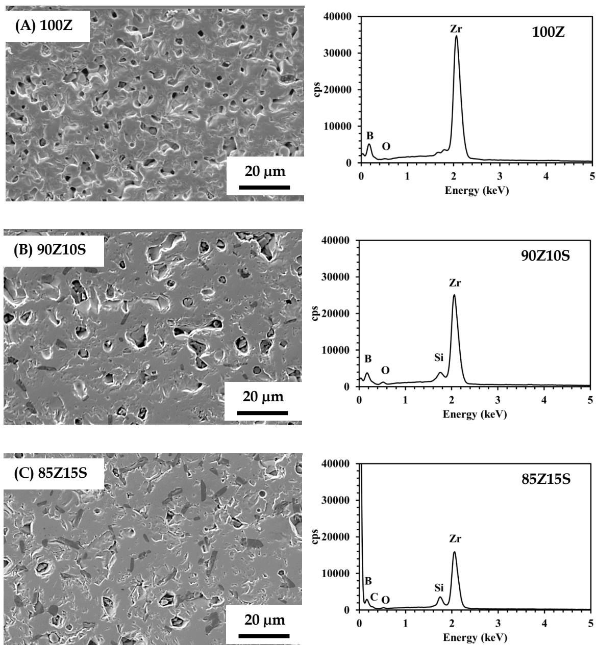
Figure 5.2: SEM micrographs in secondary electron. (SE) mode and EDS spectrums of sintered pellets at 2100 ^{\circ}\text{C} (1000 \times ). (A) 100Z, (B) 90Z10S, (C) 85Z15S, (D) 80Z20S, (E) 75Z25S and (F) 70Z30S.
