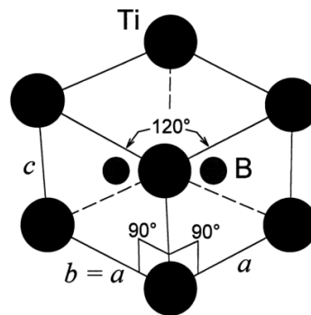
Figure 1.10: The hexagonal unit cell of single crystal \text{TiB}_2 (Munro 2000).
